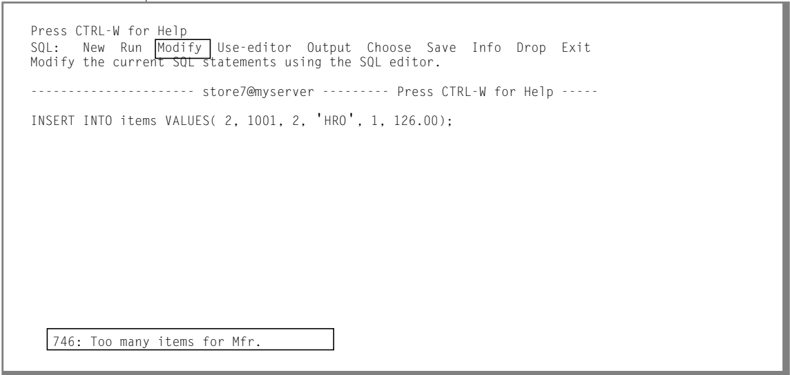
Figure 11-3 Error Number -746 with User-Specified Message Text
