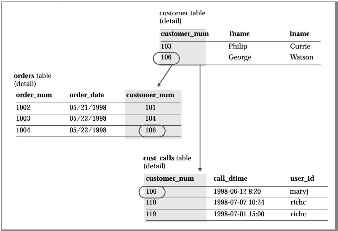
Figure 6-4 Referential Integrity in the Demonstration Database
