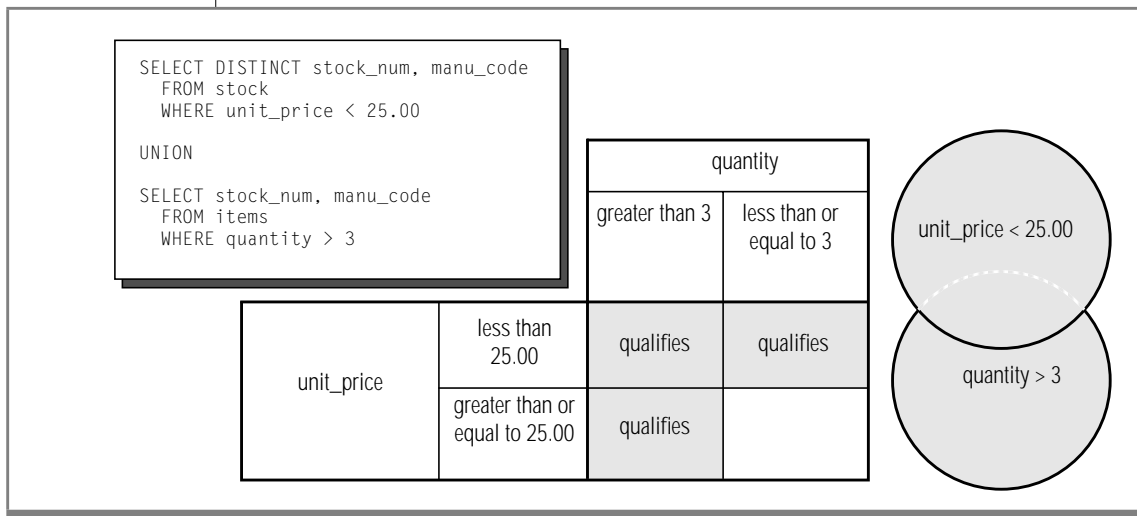
Figure 5-1 The Union Set Operation
