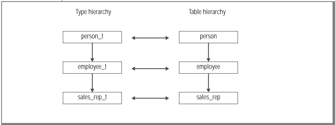
Figure 3-5 Type and Table Hierarchies
