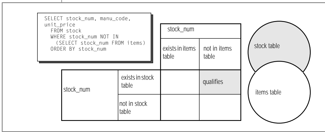
Figure 5-3 The Difference Set Operation
