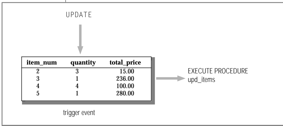
Figure 11-1 Trigger Event and Triggered Action
